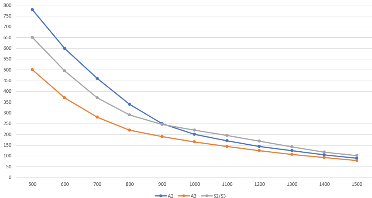
Load capacity (Kg) for A2/A3 and S2/S3 Alminor Shelves 500-1500mm @ 0,5% deflection
